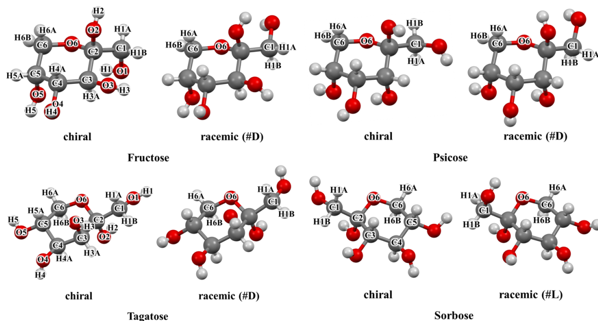
Figure 2. Numbering of ketohexoses.
