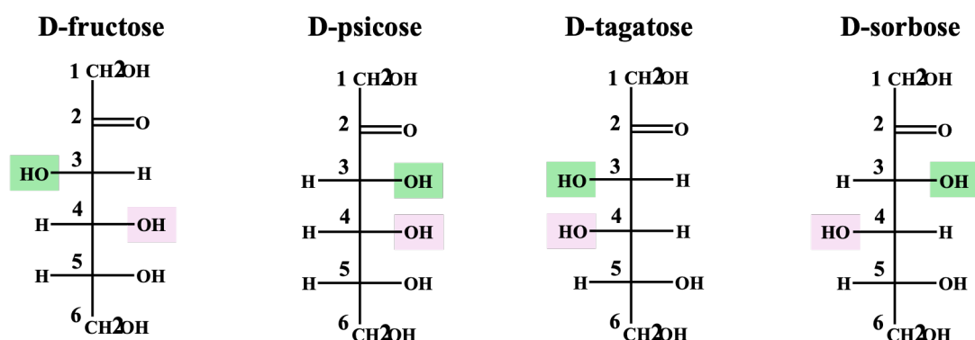
Figure 1. Fischer projections of ketohexoses.
