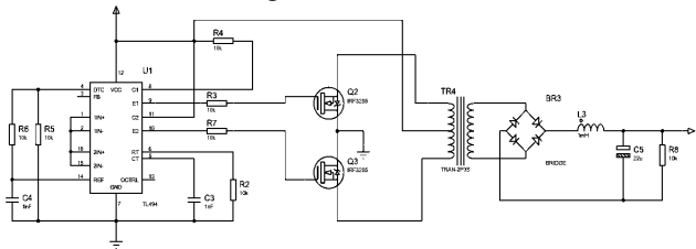
Gambar 3.4 Skematik DC to DC converter
